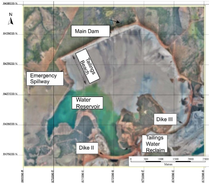
Figure 1: Chapada Tailings Storage Facility Layout
